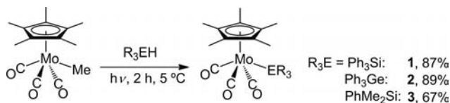
Scheme 1. Synthesis of the silyl- and germyl-molybdenum complexes.
