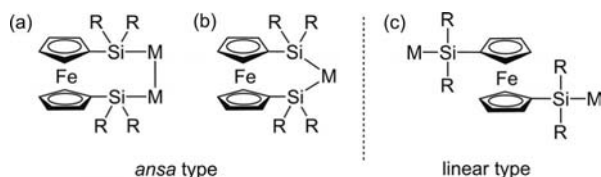
Figure 1. Two types of groups for the 1,1'-bis(silyl)ferrocenylene complex that has two M–Si bonds.
