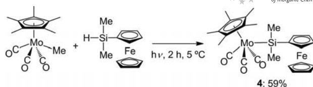
Scheme 2. Reaction of [\text{Cp}^*\text{Mo}(\text{CO})_3(\text{Me})] with (dimethylsilyl)ferrocene.
