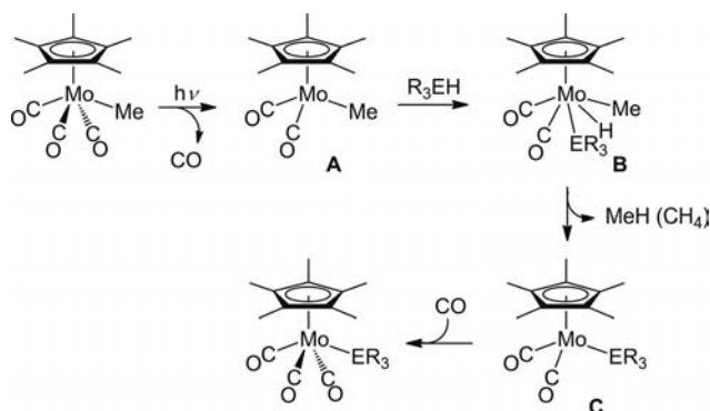
Scheme 4. Proposed mechanism of demethanative Mo–E ( \text{E} = \text{Si}, \text{Ge} ) bond formation.
