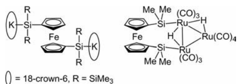
Figure 4. Two types of 1,1'-bis(silyl)ferrocene complexes with metal–silicon bonds that were previously reported.
