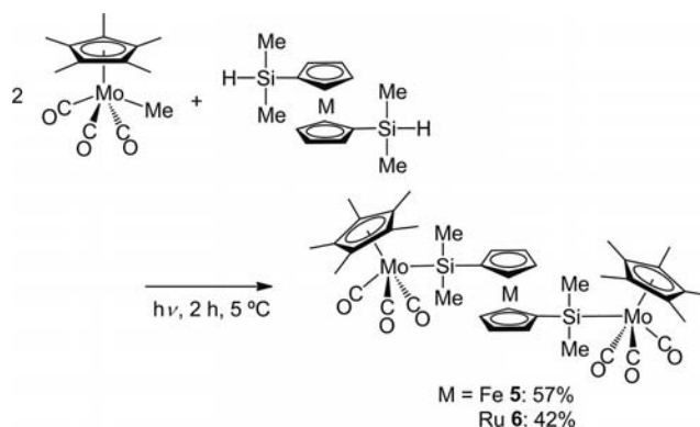
Scheme 3. Reaction of [\text{Cp}^*\text{Mo}(\text{CO})_3(\text{Me})] with the metallocenes that have one or two dimethylsilyl group(s).
