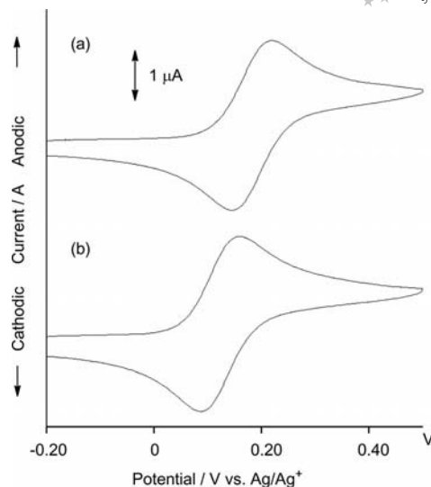
Figure 5. Cyclic voltammograms of (a) 0.5 mM of 4 at 25 °C and (b) 0.5 mM of 5 at 25 °C in a CH 2 Cl 2 solution that contains n Bu 4 NPF 6 (0.10 M) (scan rate = 0.1 V s –1 ); E_{1/2} = 0.18 V for 4 and 0.12 V for 5 .
