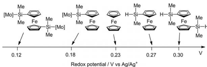
Figure 6. Redox potentials of ferrocene and the derivatives with one or two HSiMe 2 or {Cp*Mo(CO) 3 (SiMe 2 )} substituent(s); [Mo] = [Cp*Mo(CO) 3 (SiMe 2 )].
