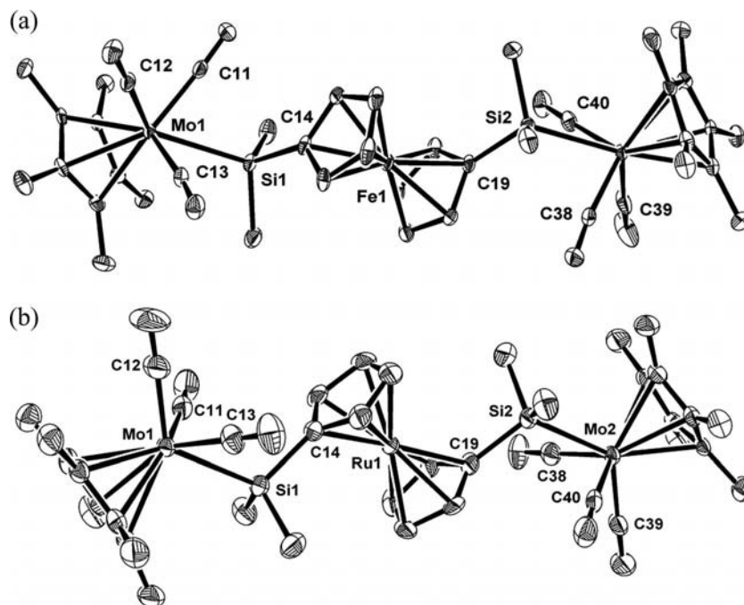
Figure 3. ORTEP drawings of 5 (a) and 6 (b) with 50% thermal ellipsoidal plots; hydrogen atoms were omitted for simplicity.
