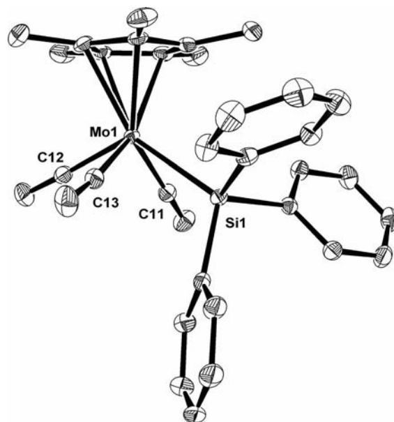
Figure 2. ORTEP drawing of the Mo1 molecule of 1 with 50% thermal ellipsoidal plots; hydrogen atoms were omitted for simplicity.
